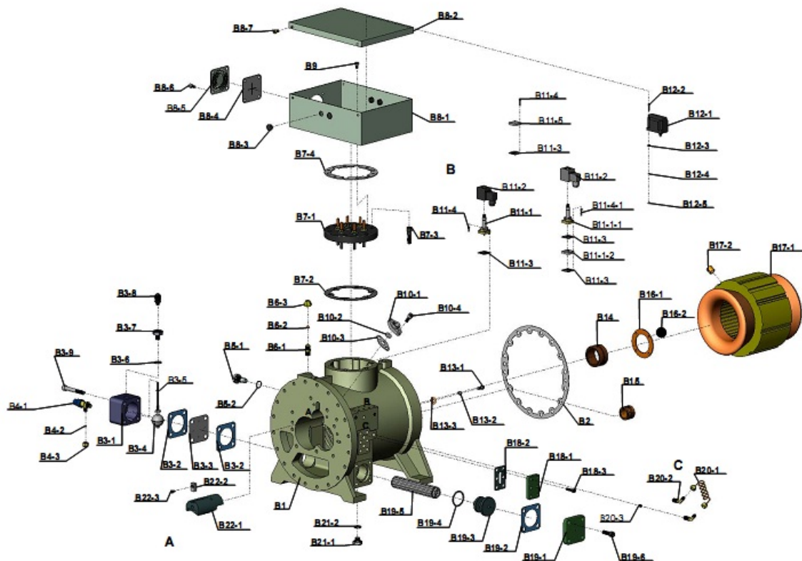
RC2-100,140,180 B - Compression Casing
